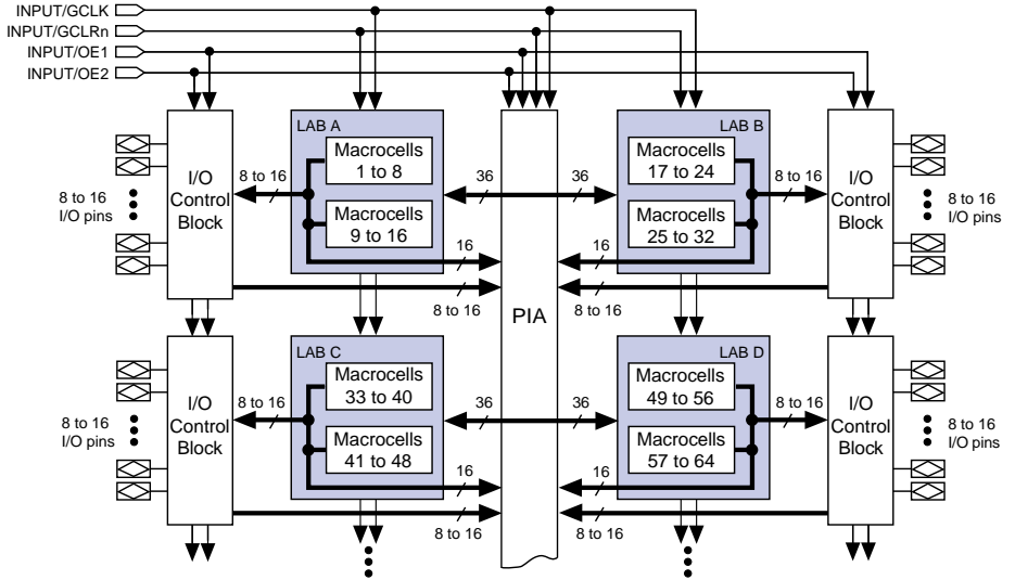
Figure 1. EPM7032, EPM7032V, EPM7064 & EPM7096 Device Block Diagram
