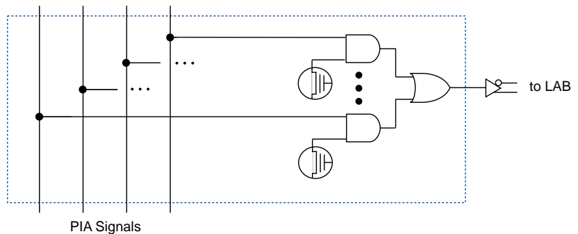
Figure 7. PIA Routing
