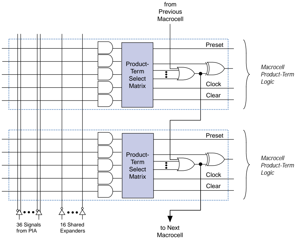
Figure 6. Parallel Expanders
