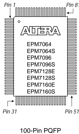
Figure 20. 100-Pin Package Pin-Out Diagram
