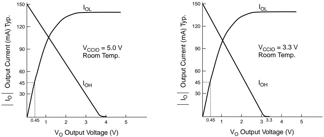
Figure 10. Output Drive Characteristics of 5.0-V MAX 7000 Devices
