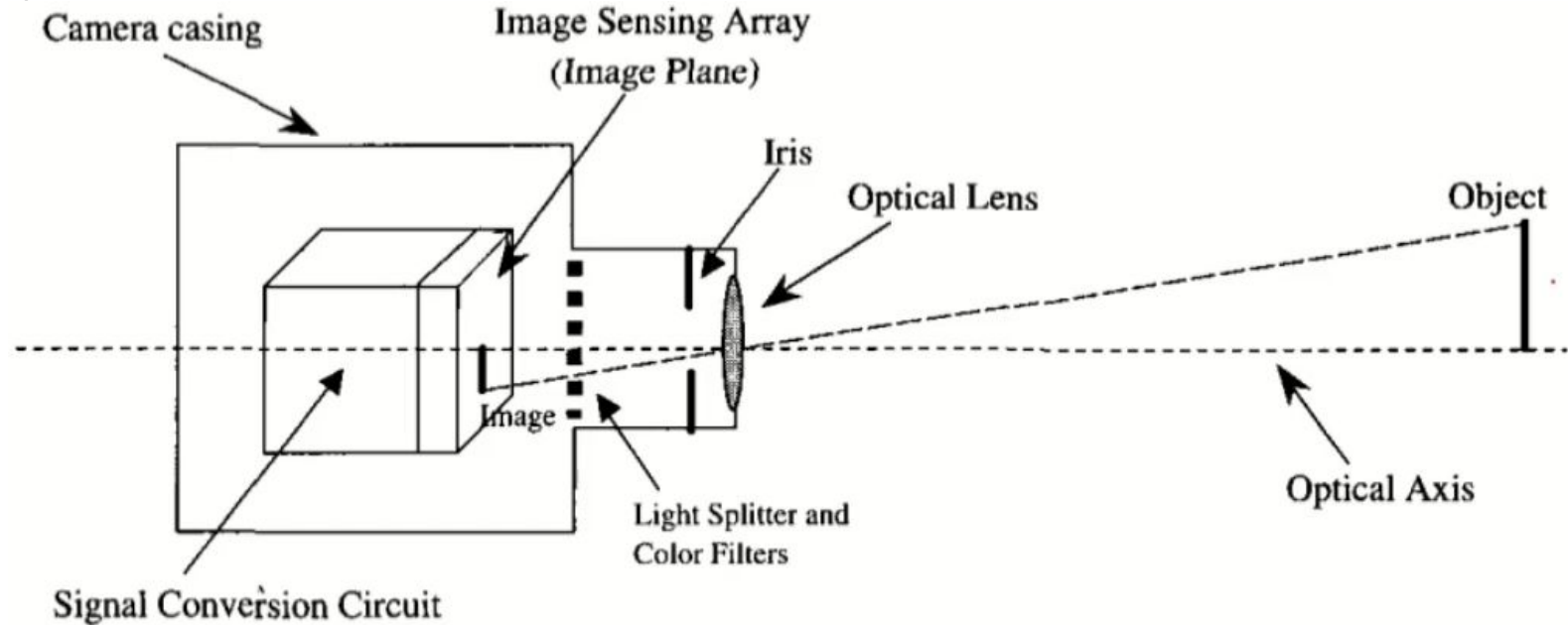
Fig. 7.10 Generic structure of an electronic camera.
