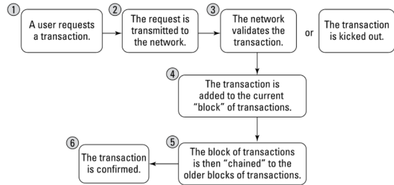
FIGURE 1-2: How blockchains work.
