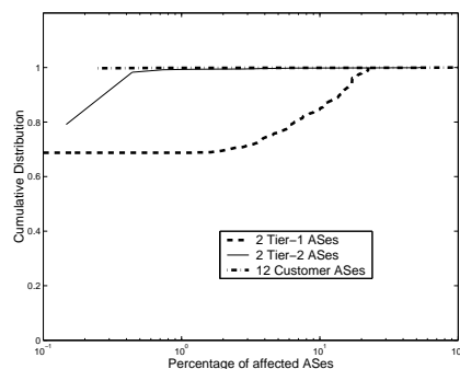
Figure 11: Effect of colluding adversaries with whisper protocols + shortest path routing
