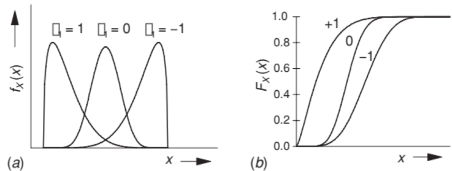
Fig. 3.2.3 Schematic diagrams of (a) the probability density functions and (b) the cumulative distribution functions of three continuous variables X with coefficients of skewness, \gamma_1 = 1, 0 , and -1 .
