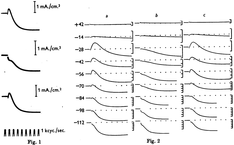
Fig. 1. Records of membrane current during 'voltage clamps' in which membrane potential was lowered by 65 mV. Top record: axon in sea water. Centre record: axon in choline sea water. Bottom record: after replacing sea water. Axon no. 15; temperature 11° C. Inward current is shown upwards in this and all other figures.
