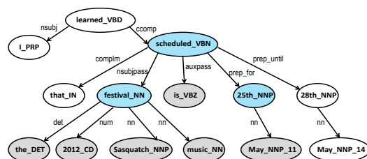
Figure 4: A sample dependency parse. The colored/greyed nodes represent all words that are extracted from the pattern {arg1} ↑subjpass↑ {rel:postag=VBN} ↓{prep_*}↓ {arg2}. The extraction is (the 2012 Sasquatch Music Festival; is scheduled for; May 25th).
