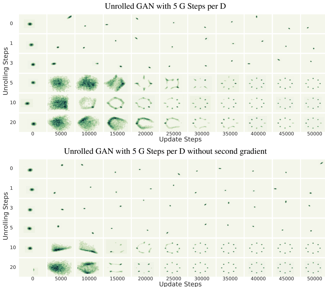
Figure App.4: Backpropagating through the unrolling process aids convergence when the discriminator does not fully converge between generator updates. When taking 5 generator steps per discriminator step unrolling greatly increases stability, requiring only 5 unrolling steps to converge. Without the second gradient it requires 10 unrolling steps. Also see Figure App.3.
