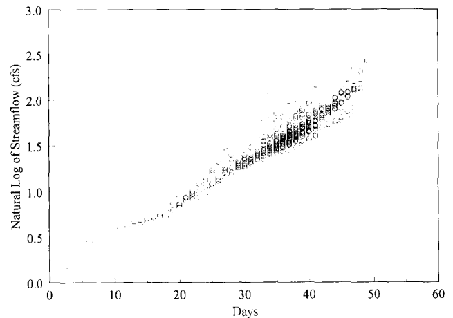
Fig. 7. Master Recession Curve for Tohickon River near Pipersville, PA (drainage area 2.52 km 2 ). The automated MRC (23 base flow days) underpredicts the manual technique (28 base flow days) by 18 percent. Note the small gaps which are the result of no data. The model projects the start of the next value following the gap by linear regression.
