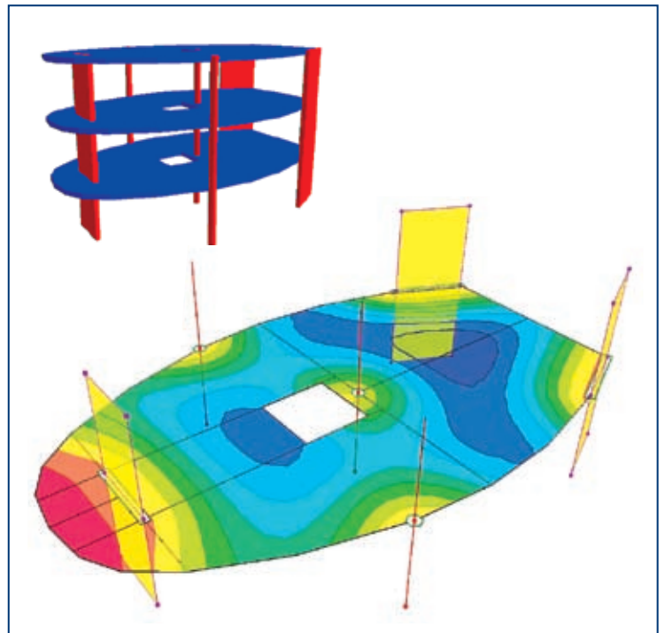
Prediction of slab deflection using an FE analysis program
