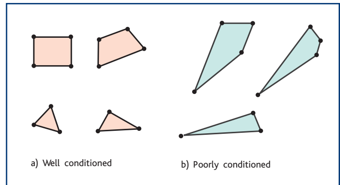
Figure 6 Element shape
