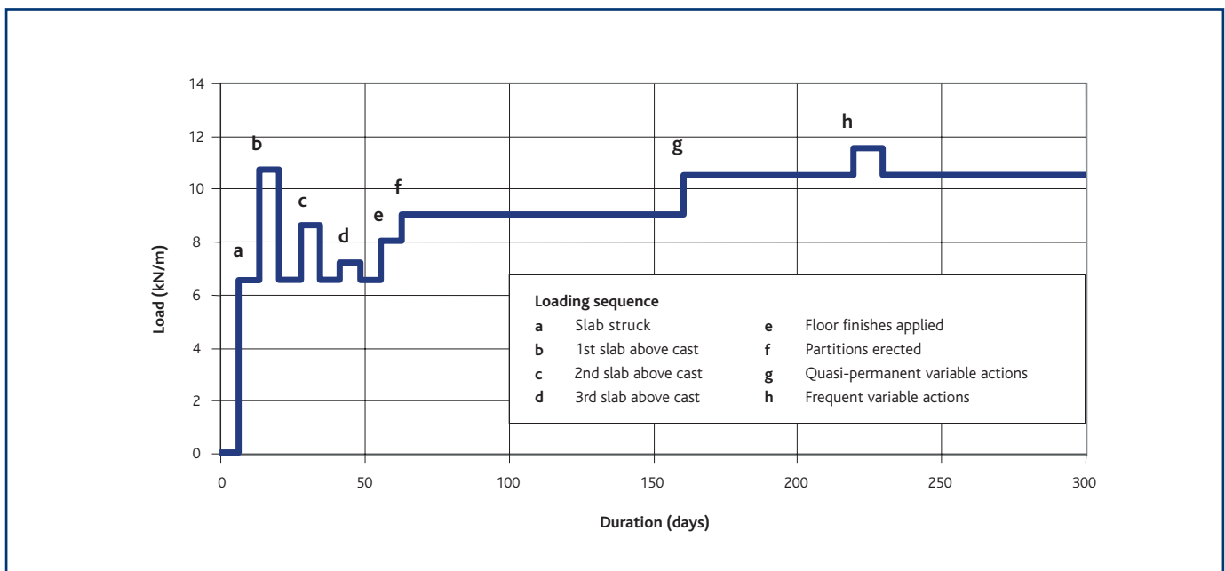
Figure 2 Loading history for a slab
