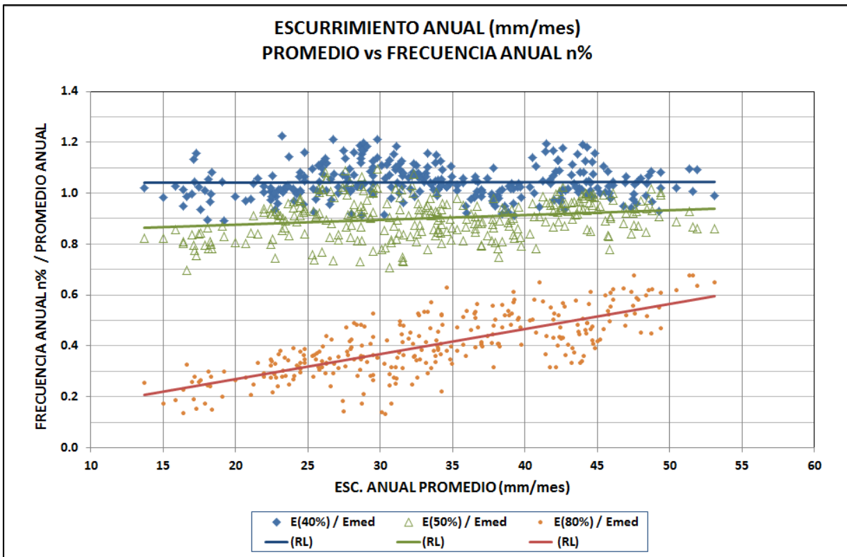
Figura 7 - Relación E_{med} vs. E_{(40\%)} , E_{(50\%)} , E_{(80\%)}
