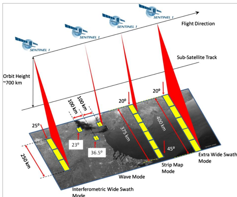
Figure 1: SENTINEL-1 Modes
