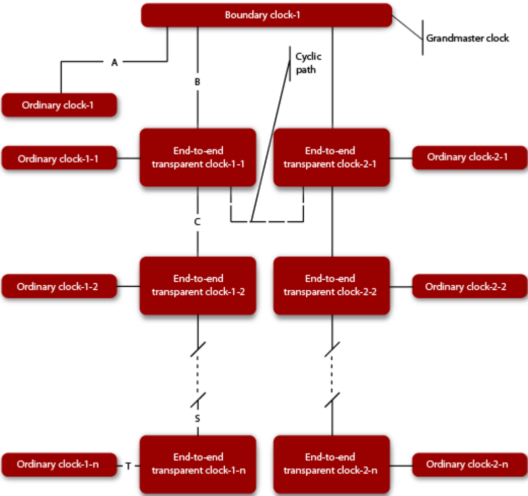
Figure 7 – Linear Topology
