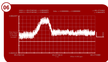
Asymmetry in Path Delay
