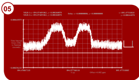
Round Trip Delay Variation
