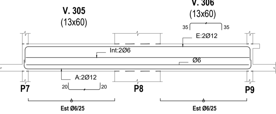
V. 305-306 Escala 1/50
