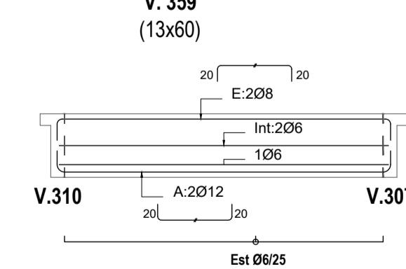
V. 359 Escala 1/50
