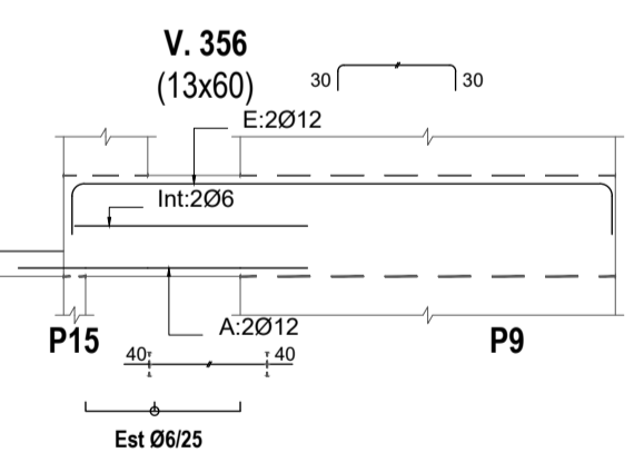
V. 356 Escala 1/50
