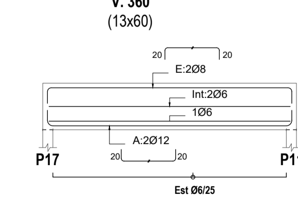
V. 360 Escala 1/50
