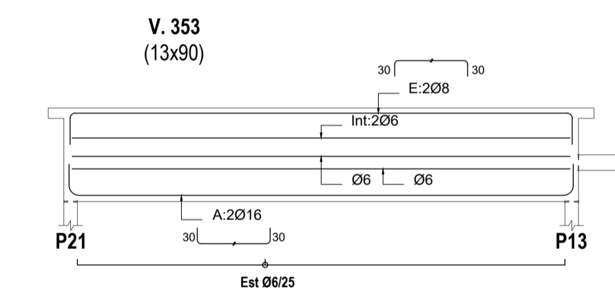
V. 353 Escala 1/50
