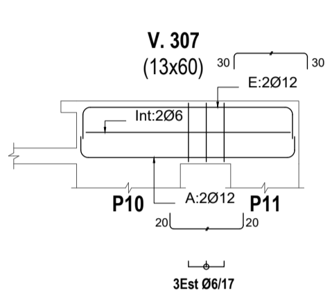
V. 307 Escala 1/50
