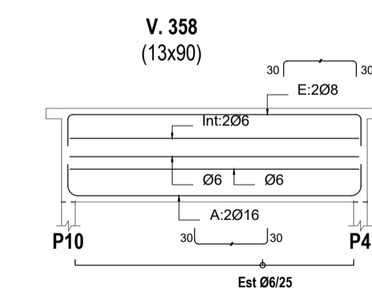
V. 358 Escala 1/50
