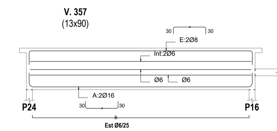
V. 357 Escala 1/50
