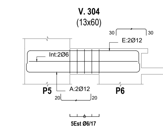
V. 304 Escala 1/50
