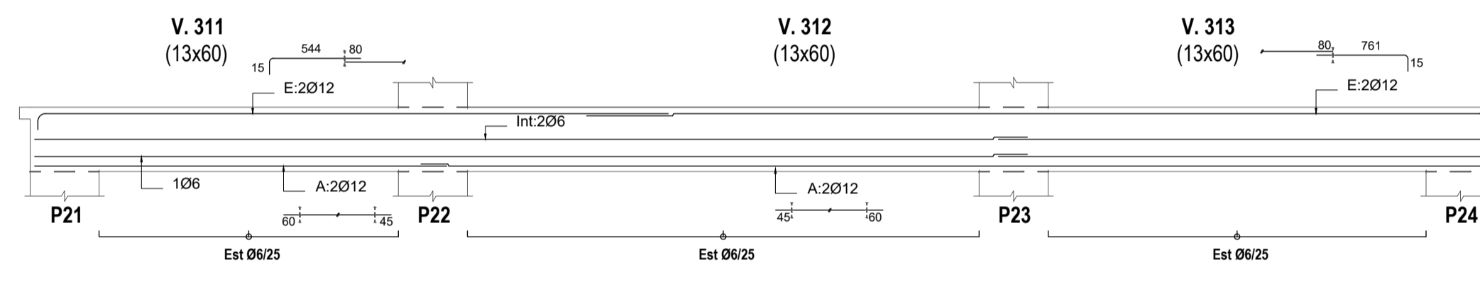
V. 311-312-313 Escala 1/50
