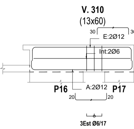
V. 310 Escala 1/50
