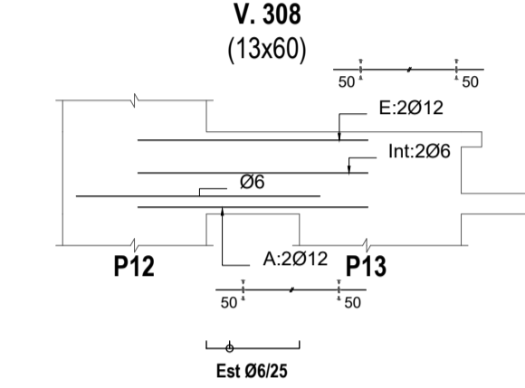
V. 308 Escala 1/50
