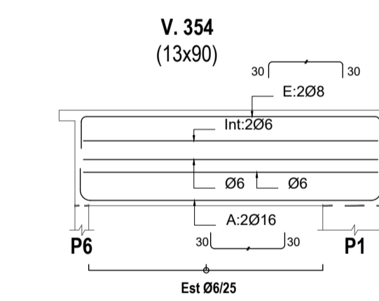
V. 354 Escala 1/50
