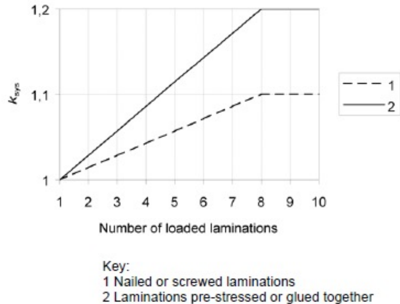
Figure 6.12 – System strength factor k_{\text{sys}} for laminated deck plates of solid timber or glued laminated members
