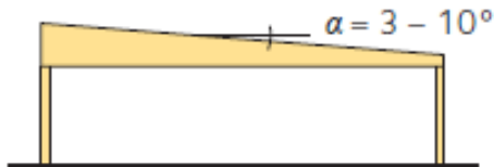
Single pitched beam
