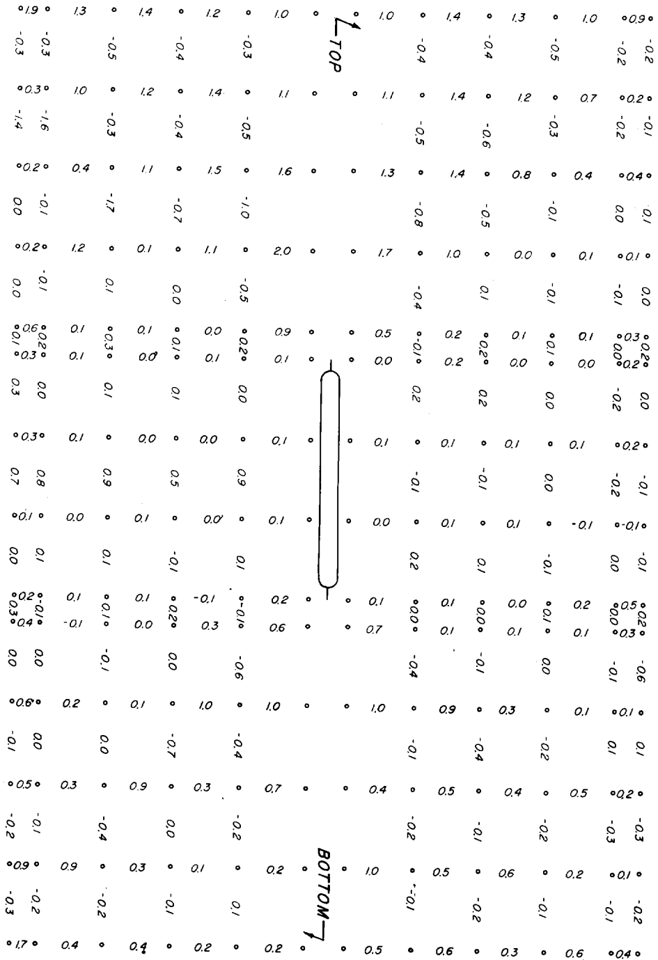
FIG. A-4 PERCENT ELONGATION PLATE A-2A (5 INCH GRID) 1/2" STEEL, 72 INCH WIDE PLATE TEMPERATURE 30-35°F NOMINAL STRENGTH 38.5 KSI 2% SHEAR
