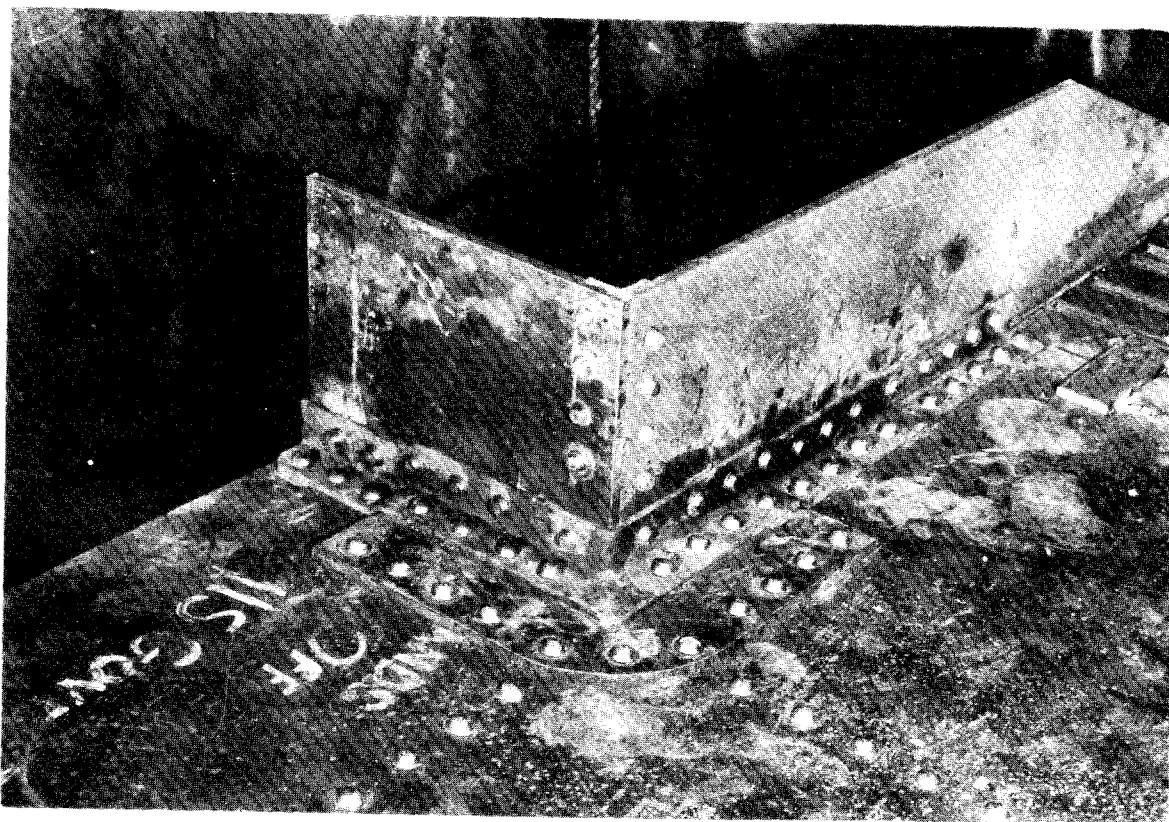
Before failure: View of corner from above deck
