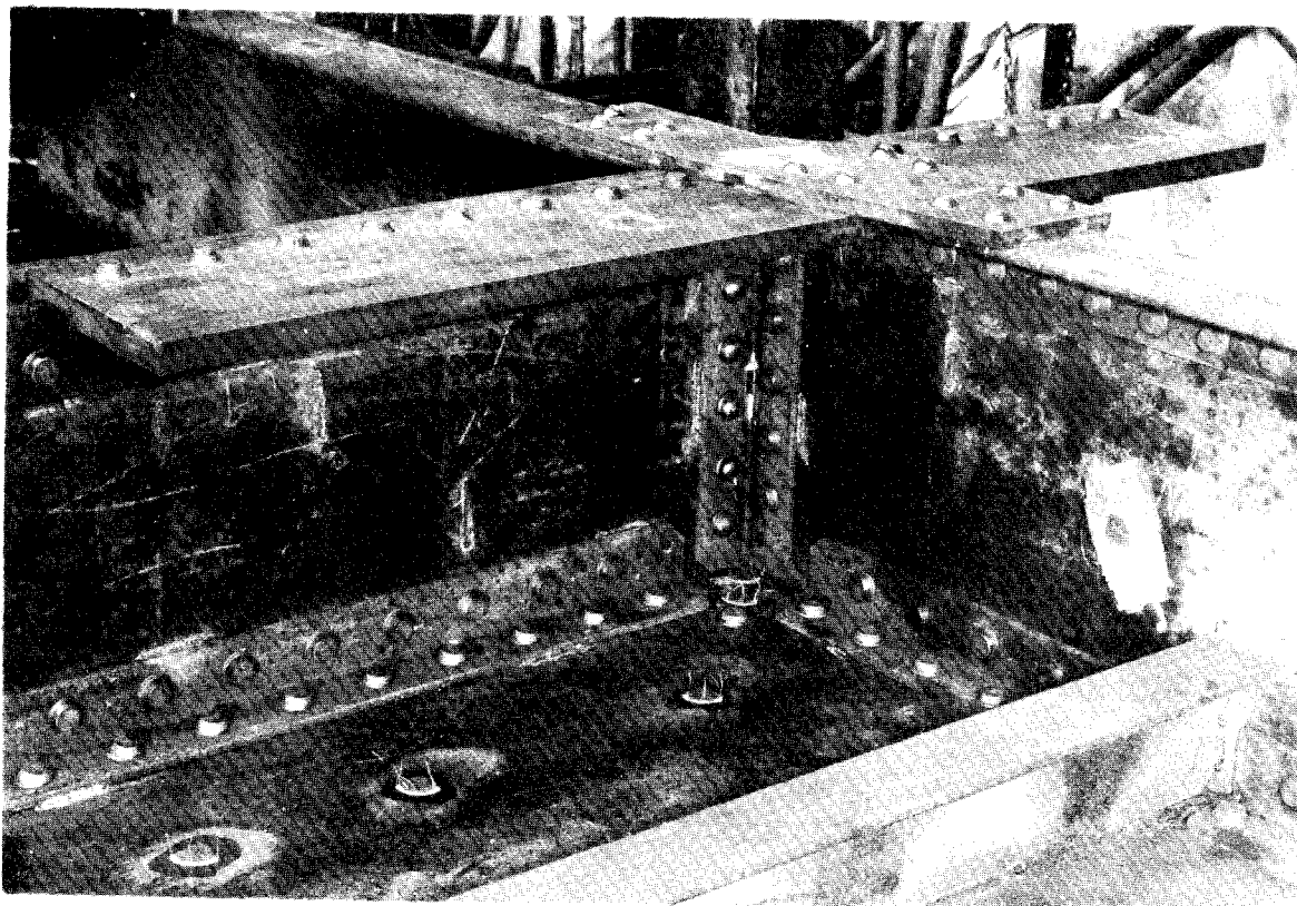
Before failure: Below deck, looking aft and inboard
