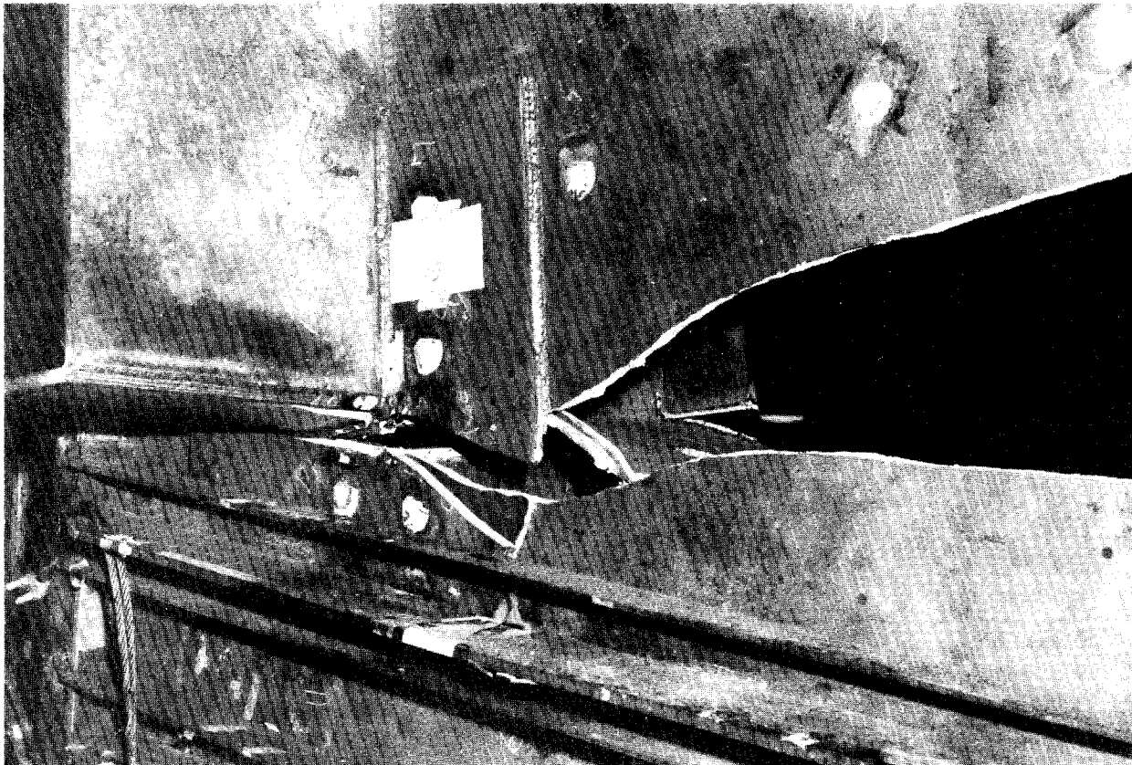
Fractures viewed from above deck
