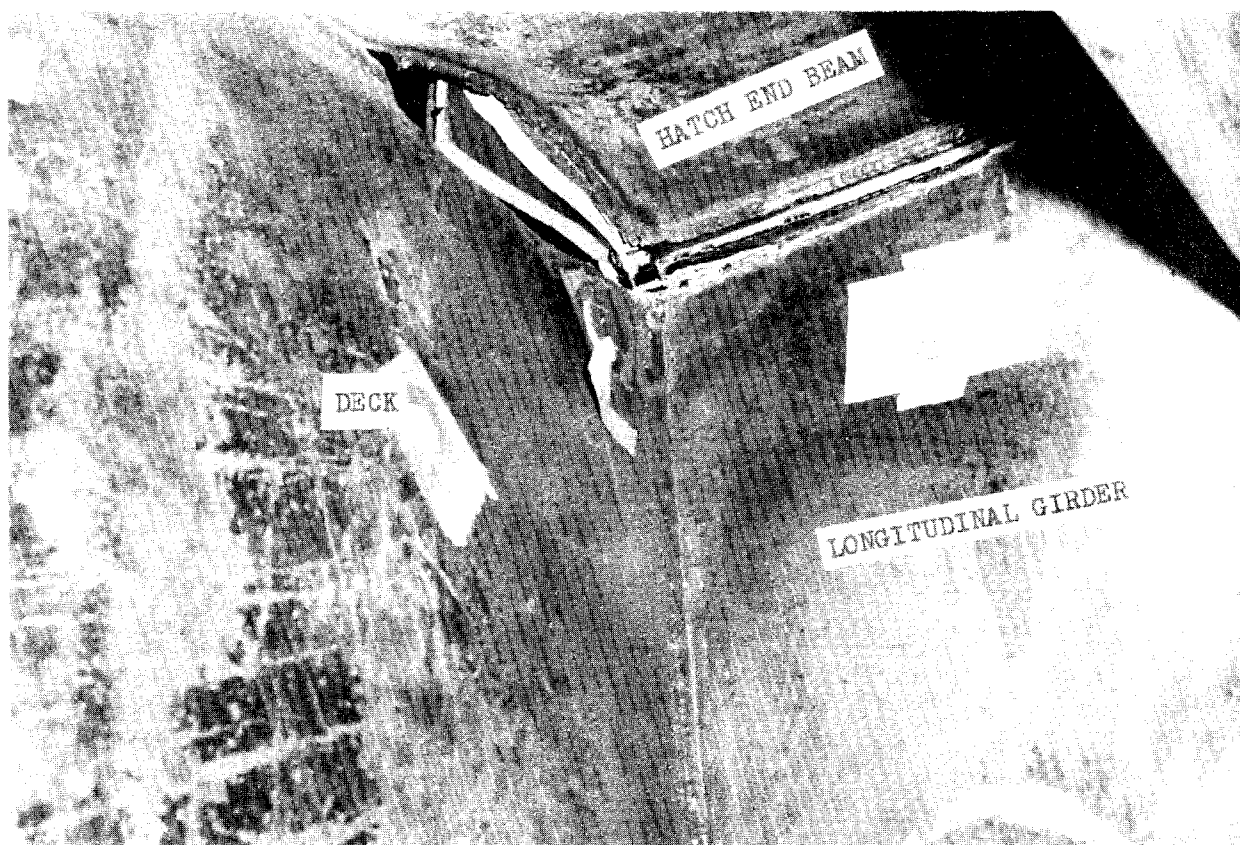
Fractures viewed from below deck, outboard and forward of hatch end beam.
