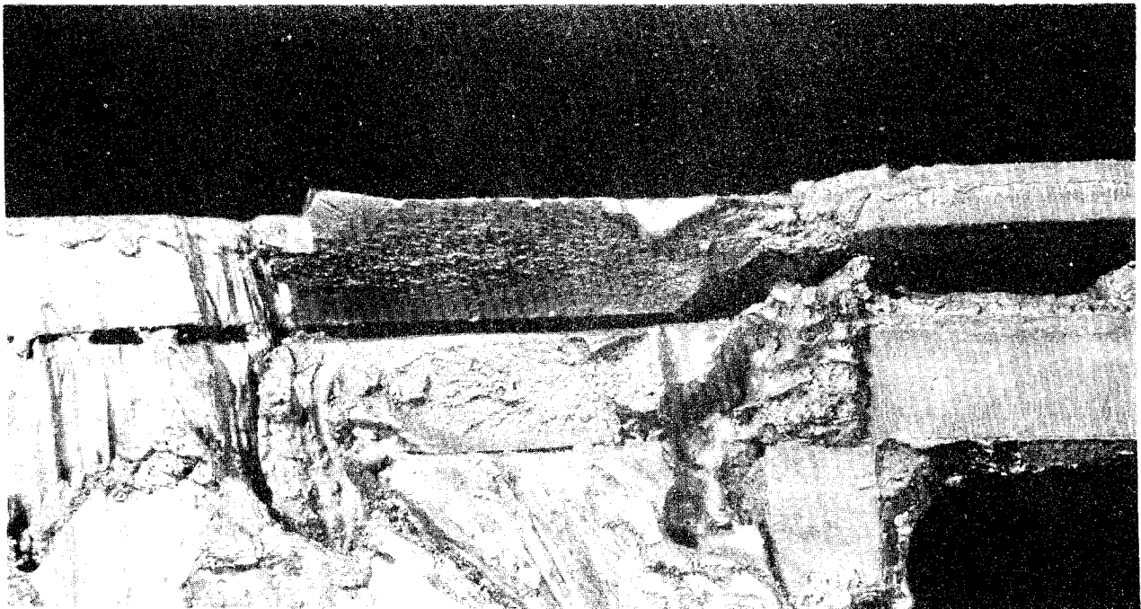
Deck and doubler fractures, looking fwd.
