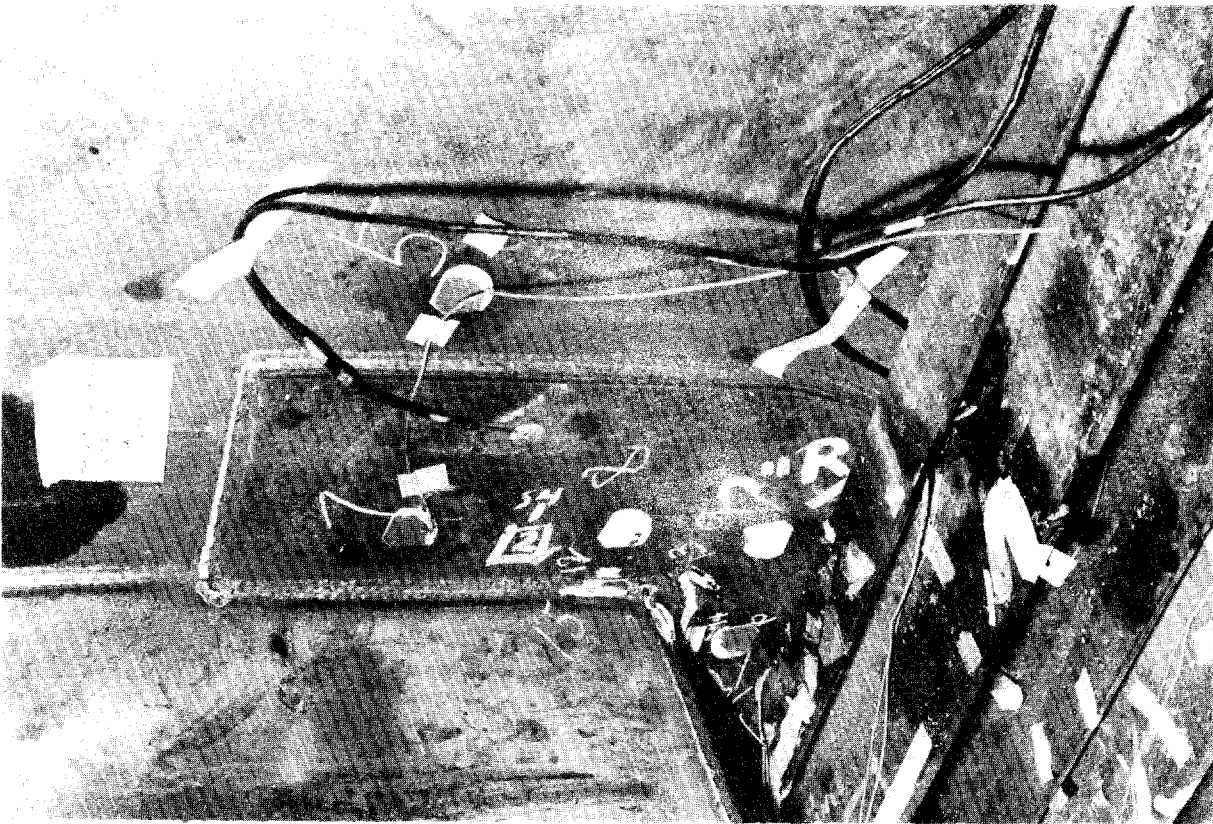
Crack in doubler-deck weld
