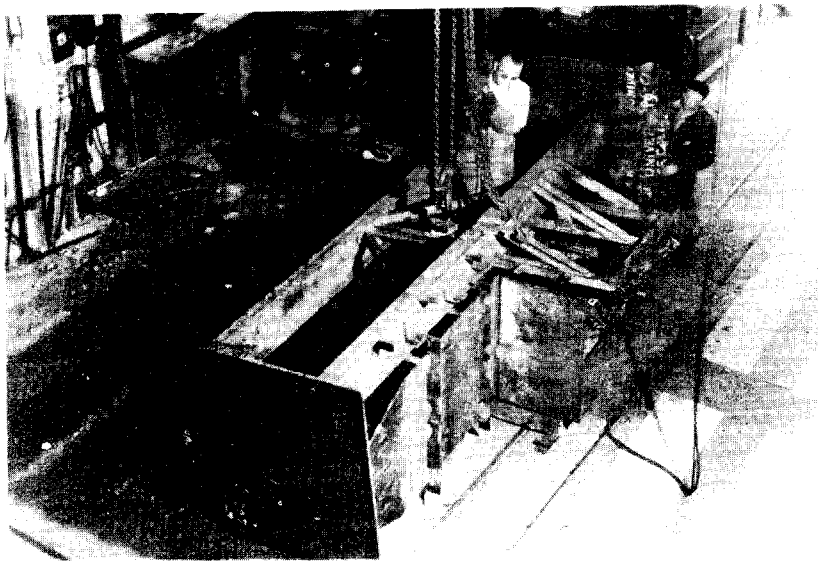
FIGURE 3 - WELDING JIG FOR FABRICATION OF HATCH CORNER SPECIMEN
