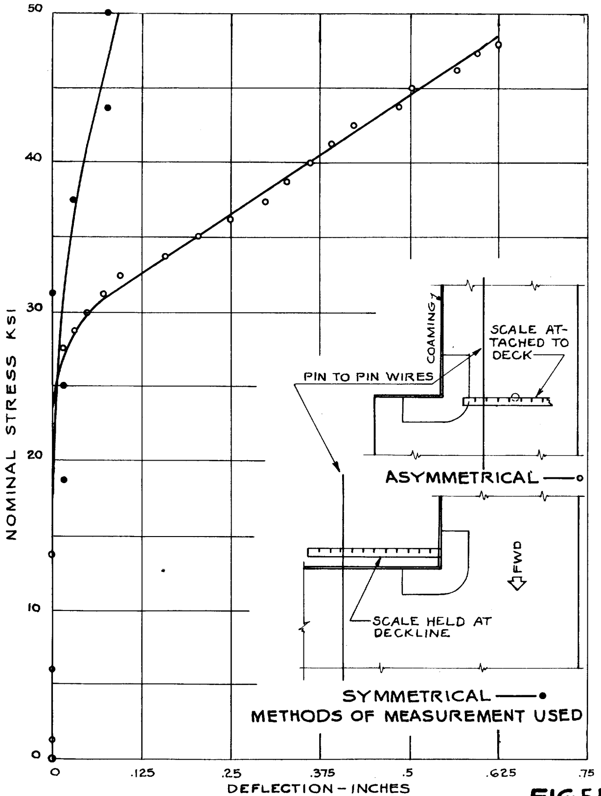
DEFLECTION MEASUREMENTS FIG.55
