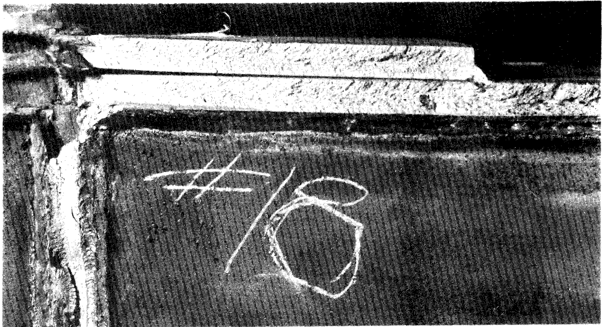
Deck and doubler fracture patterns - looking aft
