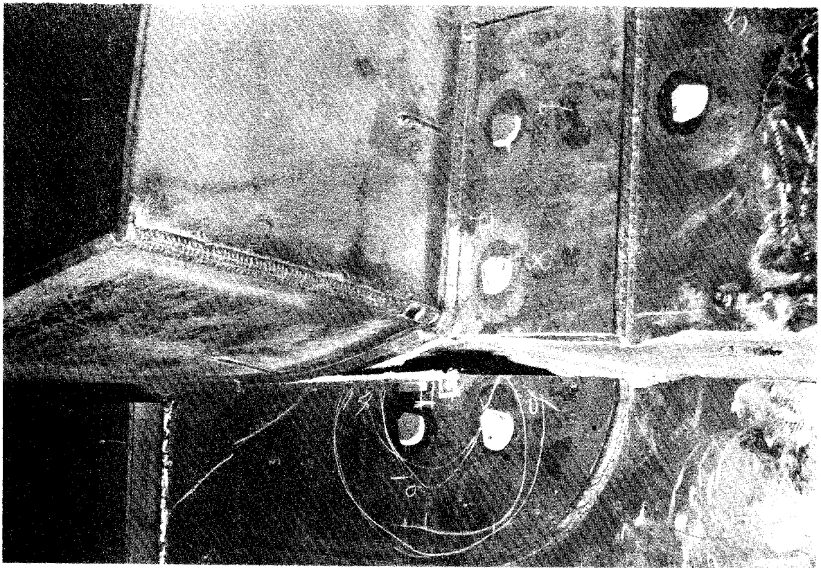
Fractures: Viewed from above deck
