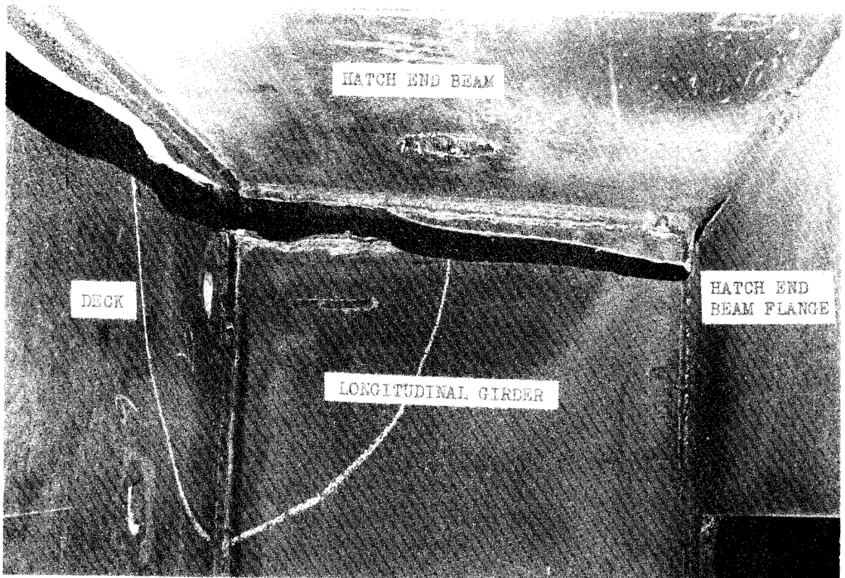
Fractures: Viewed from below deck, outboard, and fwd. of hatch end beam
