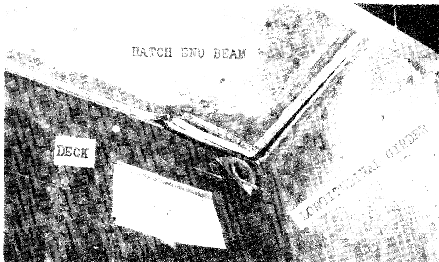
Fractures: Viewed from below deck, outboard, and fwd. of hatch end beam
