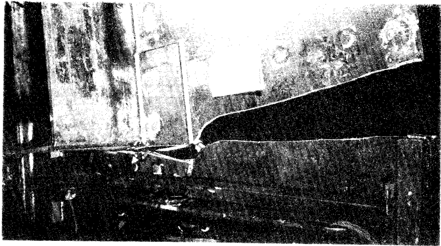
Fractures: Viewed from above deck
