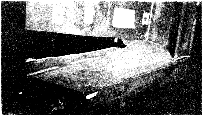
Fractures: Viewed from below deck, outboard, and aft of hatch end beam
