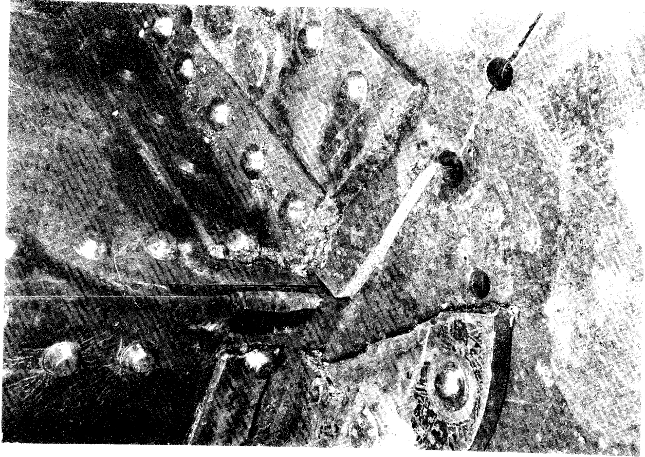
Fracture in deck (doubler cut away)
