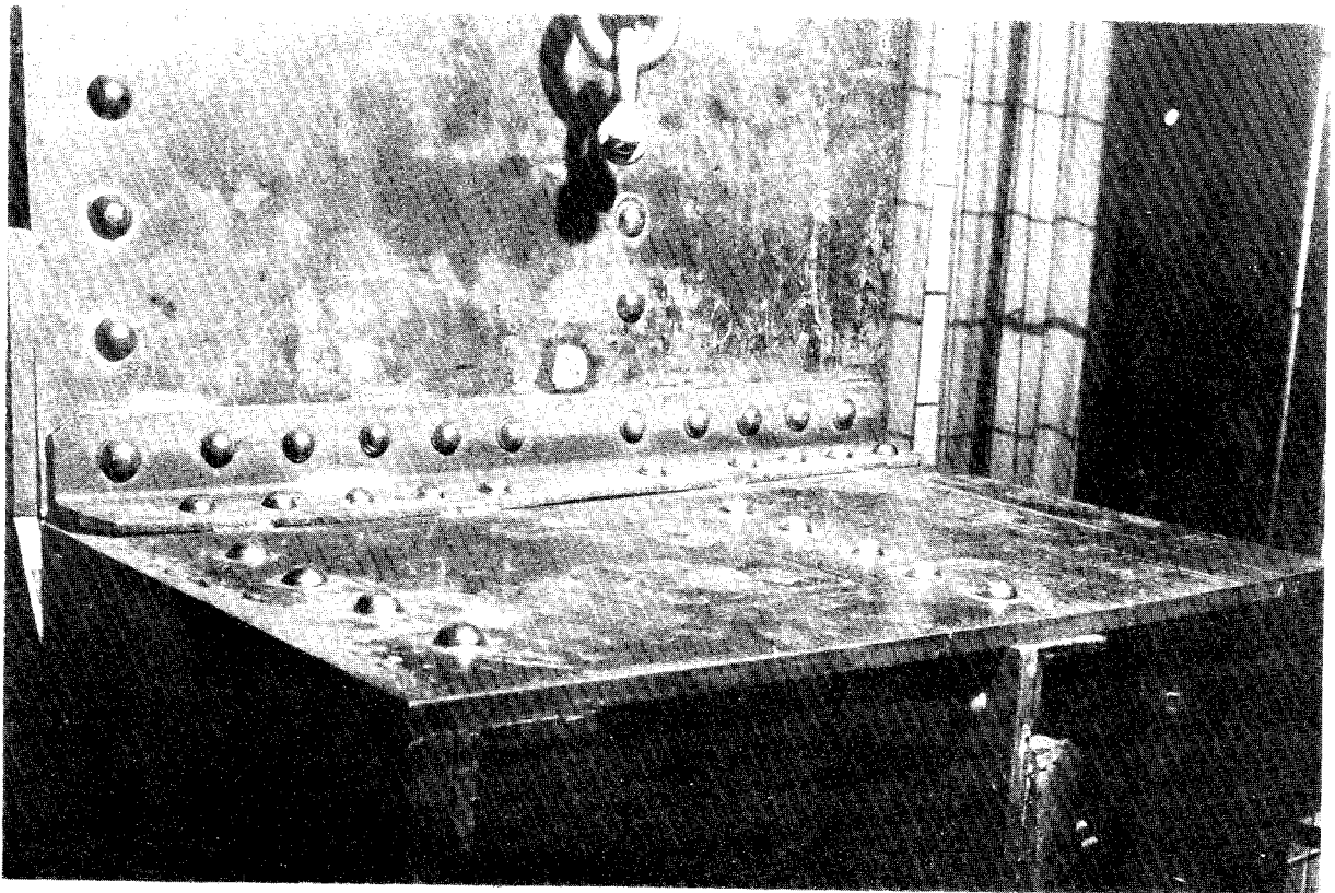
After failure: Corner viewed from inside of hatch
