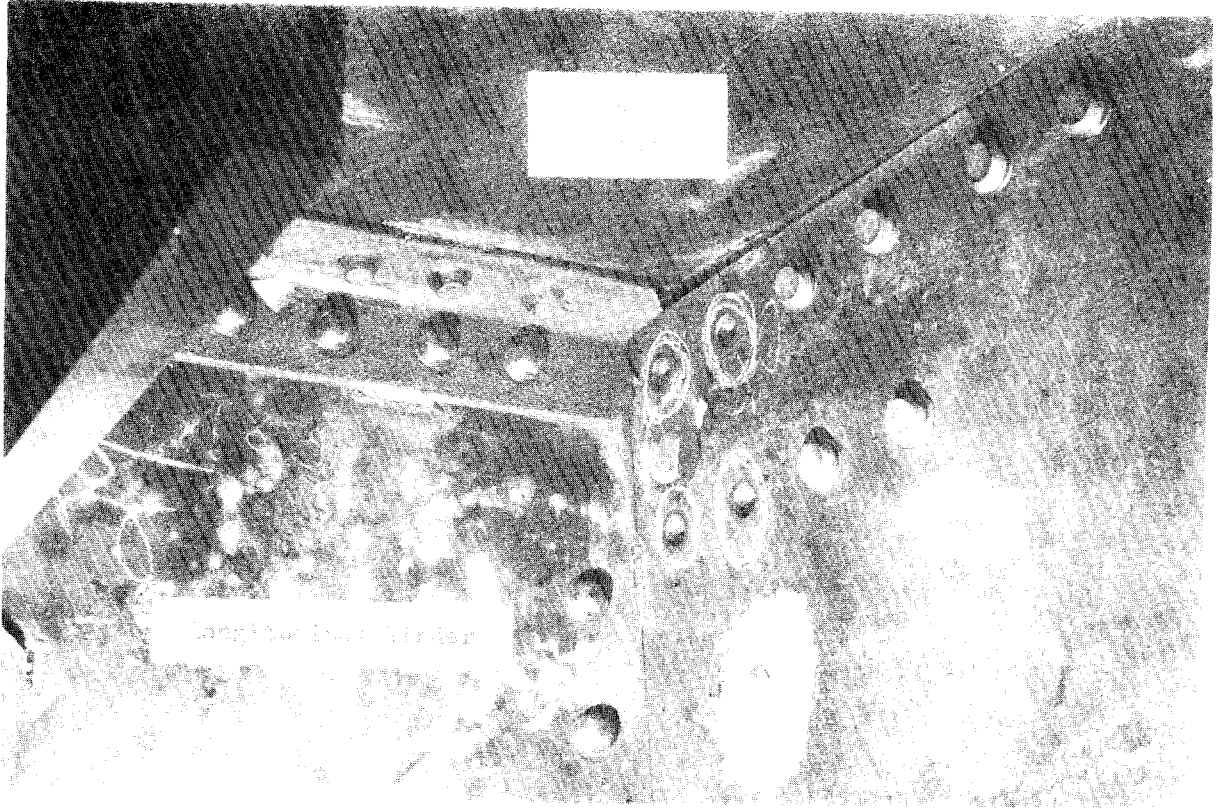
After failure: View from below deck, inboard, and fwd. of hatch end beam
