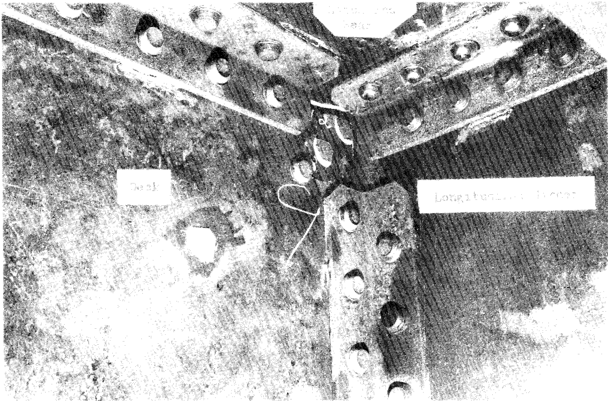
Fracture in deck: Viewed from below deck, outboard, and fwd. of hatch end beam
