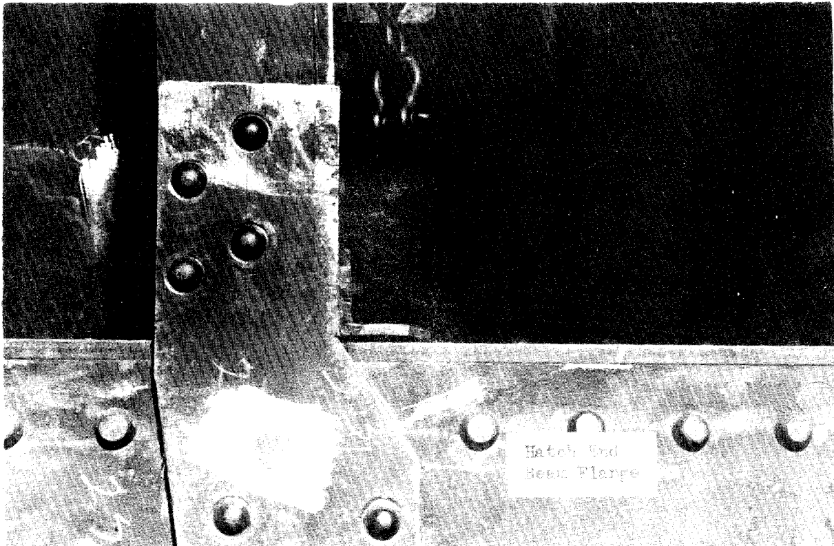
After failure: Close-up of tie-plate
