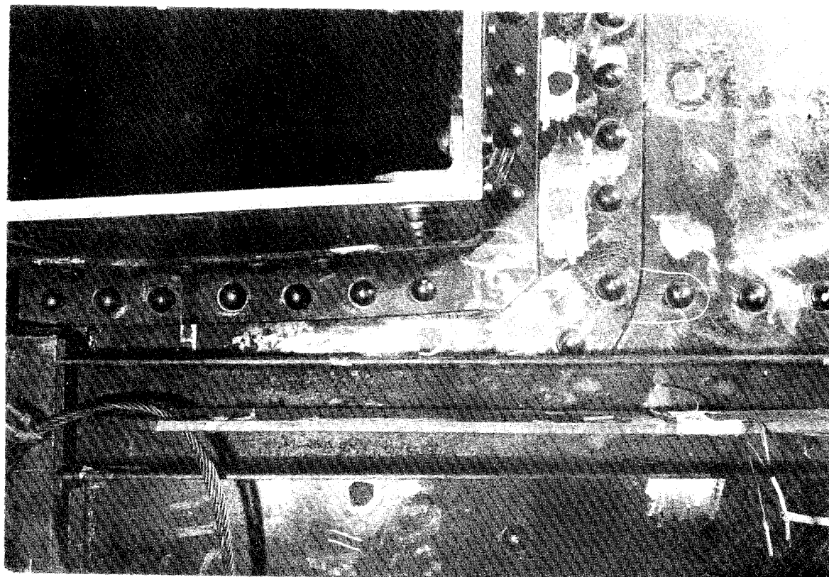
After failure: View from above deck
