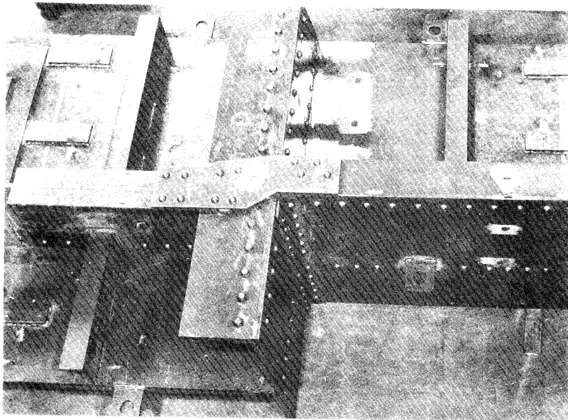
Before failure: Overall view - below deck
