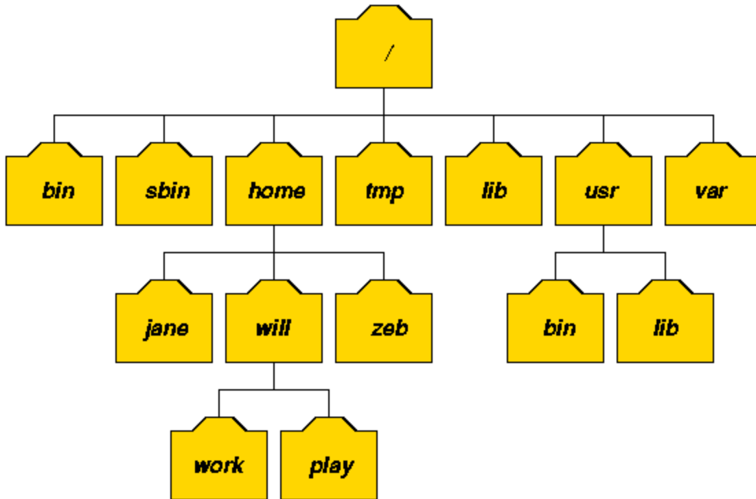
Fig. 2.1: Part of a typical UNIX filesystem tree
