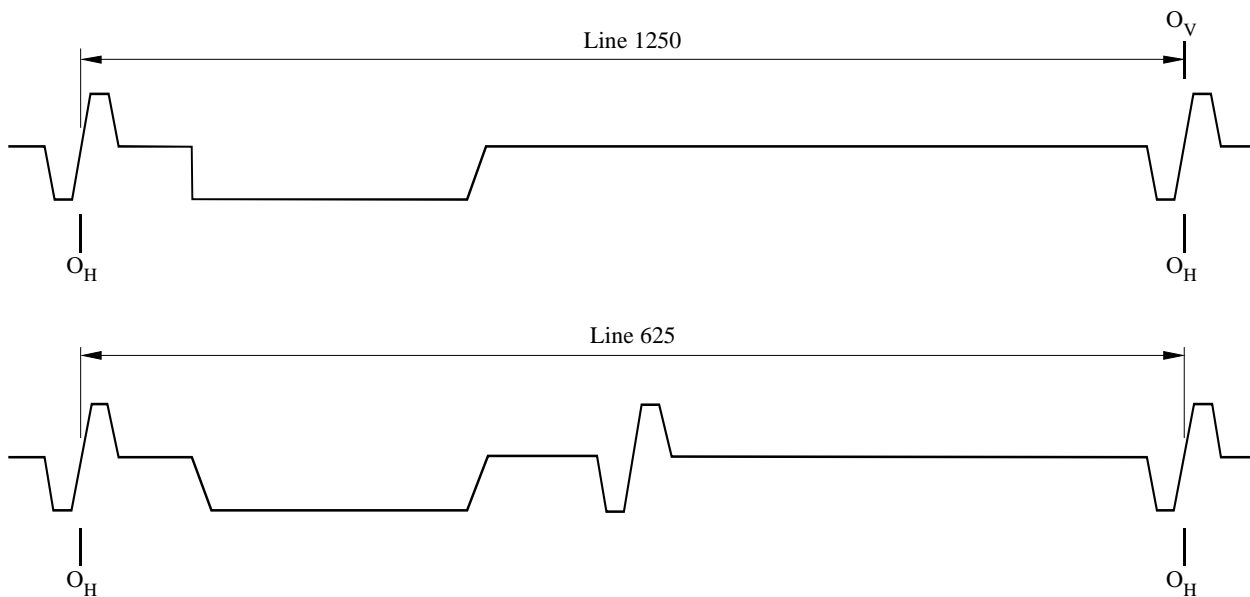
FIGURE 7 Frame and field identification for the 1250/50/2:1 system
