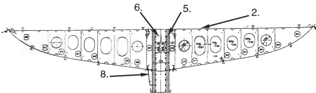
Frame at aft perpendicular (frame 0)
