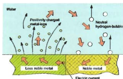
Galvanic corrosion
