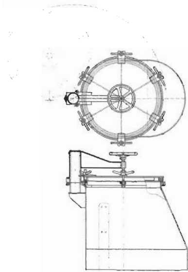
Cross section and top view of an expansion trunk with lid
