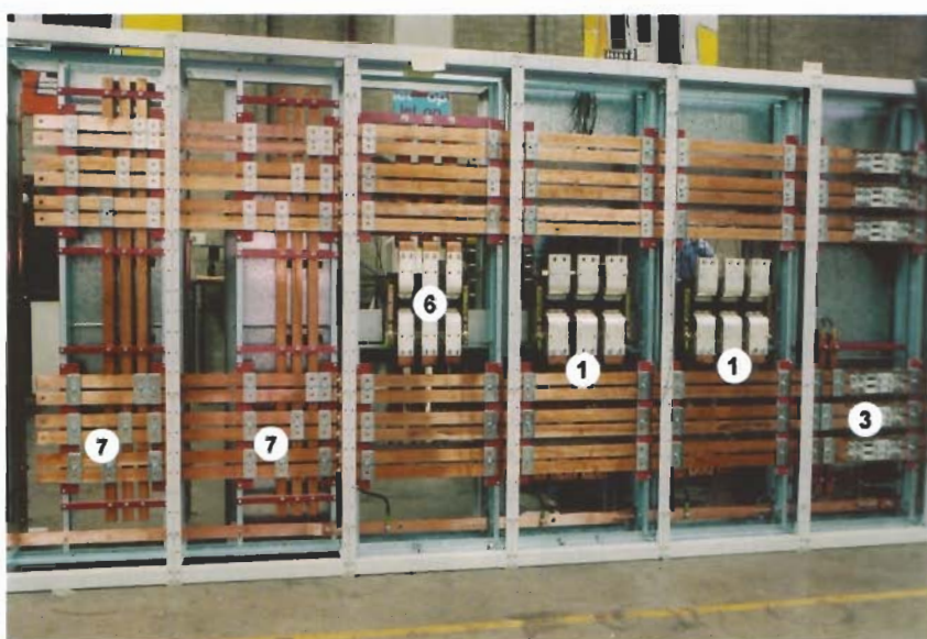
"Blue Star" main switchboard during factory testing
