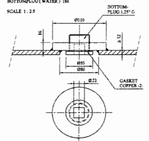
BOTTOMPLUG (WATER) 10x SCALE 1 : 2.5
