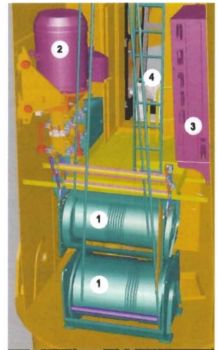
Crane house
