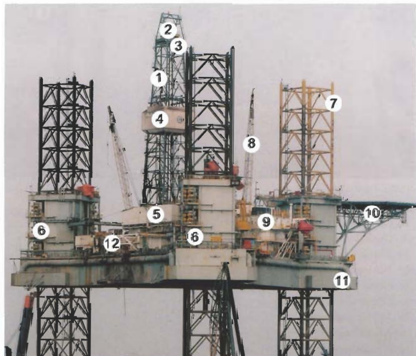
Jack-up rig in jacked up position.
