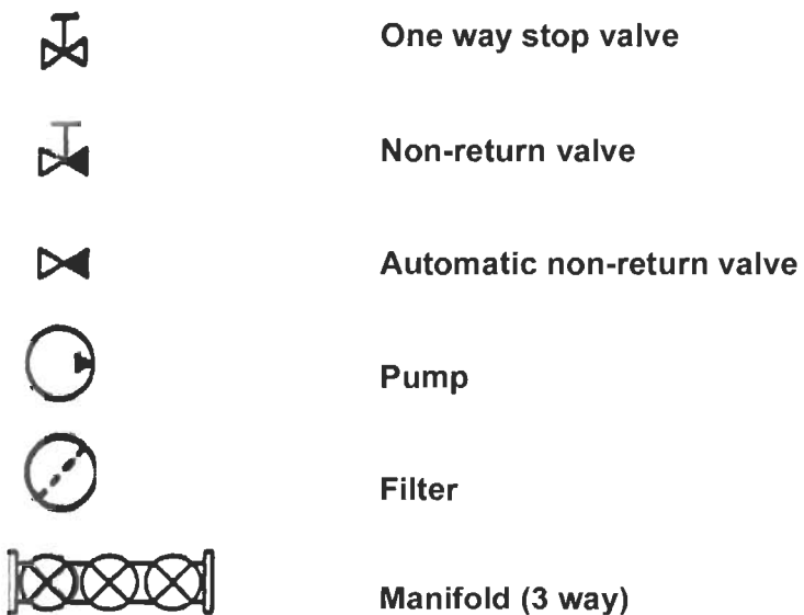
Common symbols
