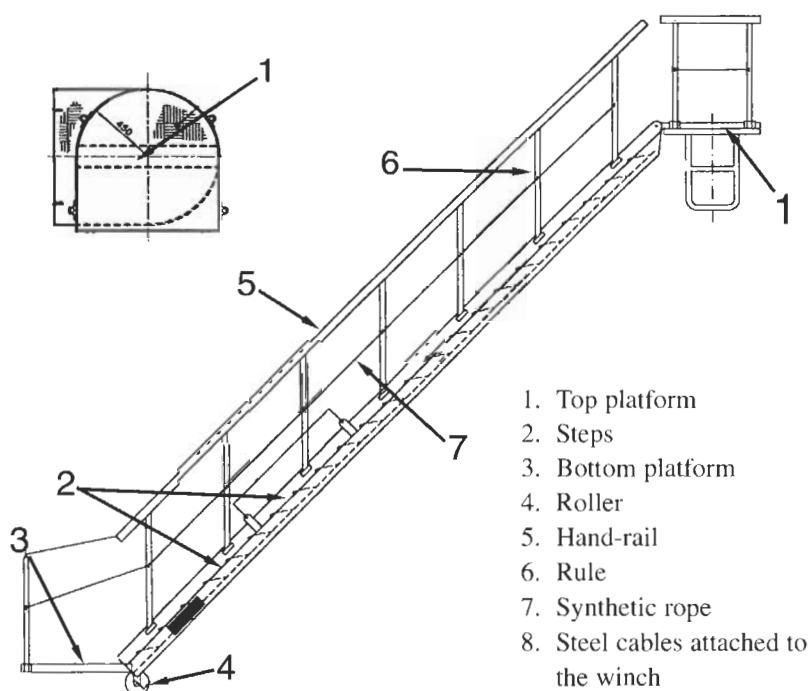
Side view of an accommodation ladder and top view of the platform:
