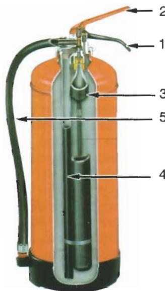
Cross-section of a powder extinguisher
