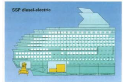
Drive via rudder propeller
