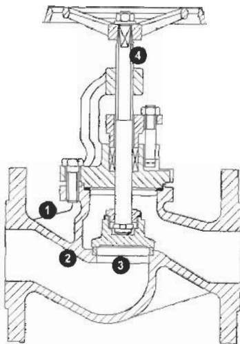
Globe valve
