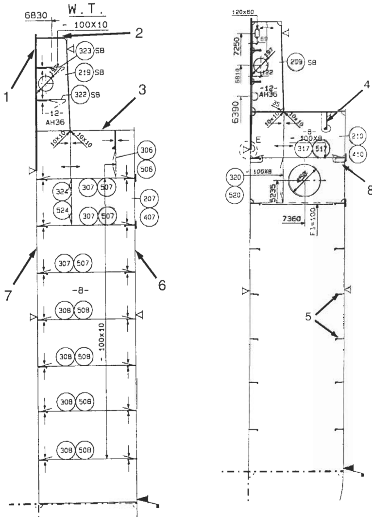
Section 1800. (2450, 3050, 3675) a.b.
