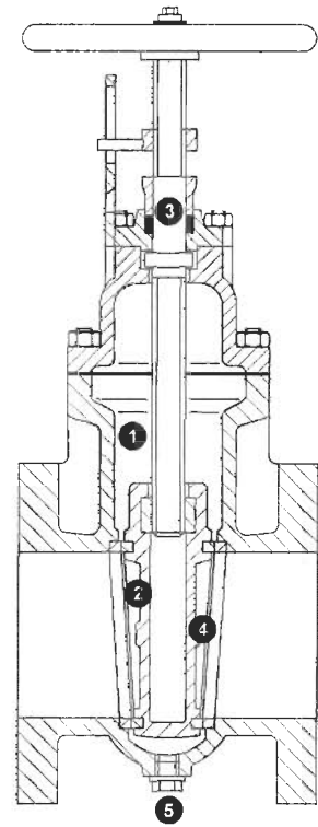
Gate valve
