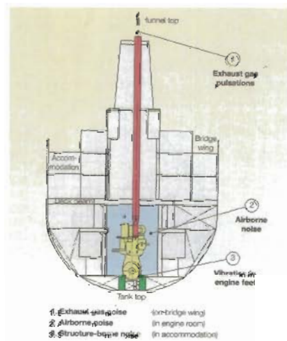
Vibration sources
