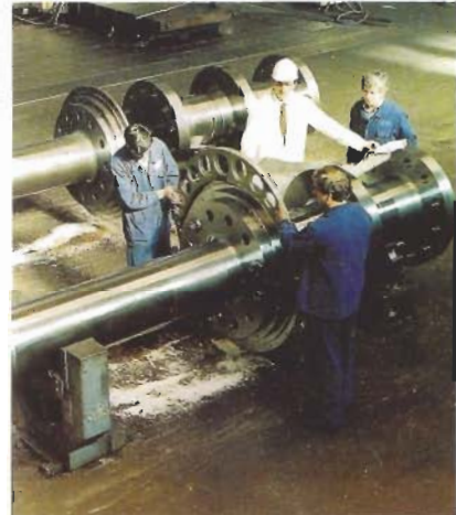
In a manufacturer's workshop a local surveyor reviews the fit-up and alignment of intermediate and thrust shafts.
