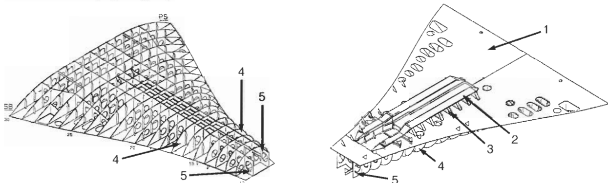
Assembly drawing
