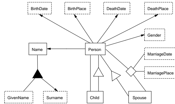
Fig. 7 Target Ontology of Desired Biographical Assertions.
