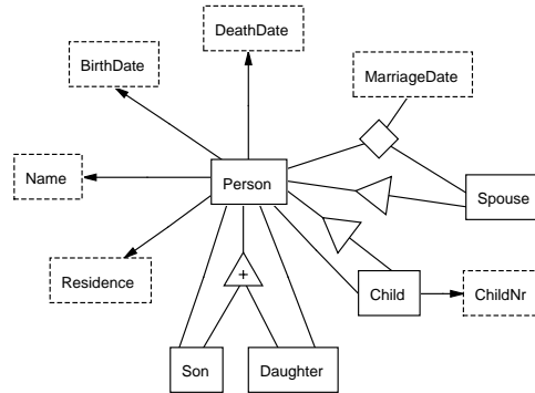
Fig. 4 Ontological Conceptualization for Assertion Extraction.
