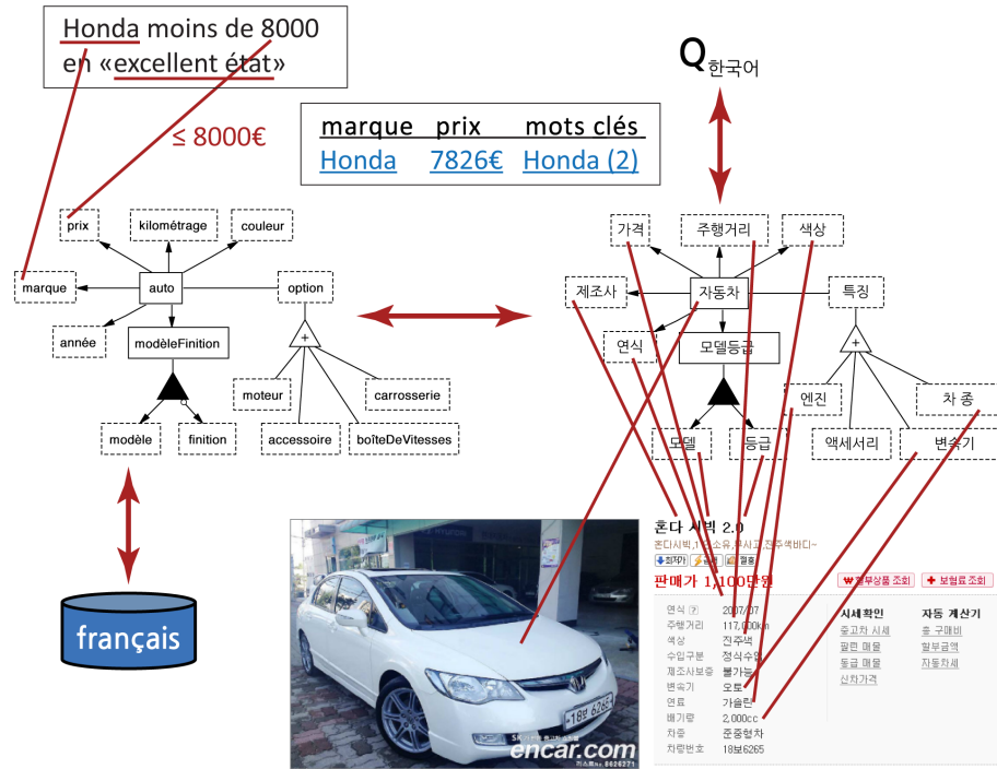
Fig. 3 Cross-Language Query Processing.
