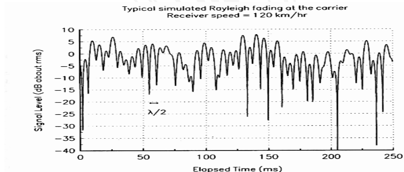
Figure 5.15 A typical Rayleigh fading envelope at 900 MHz [from [Fun93] © IEEE].
