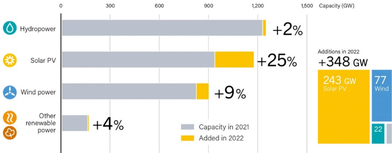
Renewable Power Total Installed Capacity and Annual Additions, by Technology, 2022
