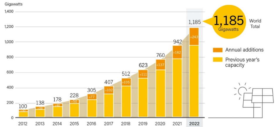
Solar PV Global Capacity and Annual Additions, 2012-2022
