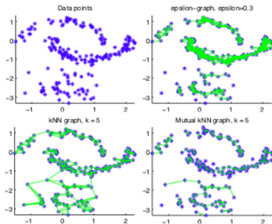
Figure: Different similarity graphs (Von Luxburg, 2007)
