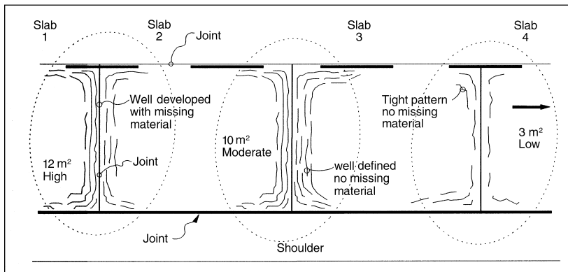
FIGURE 51 Distress Type JCP 2—“D” Cracking.
