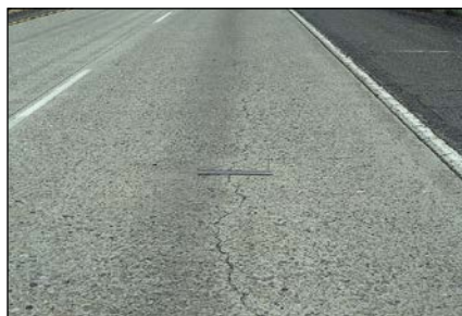
FIGURE 94 Distress Type CRCP 2—Low Severity Longitudinal Cracking.
